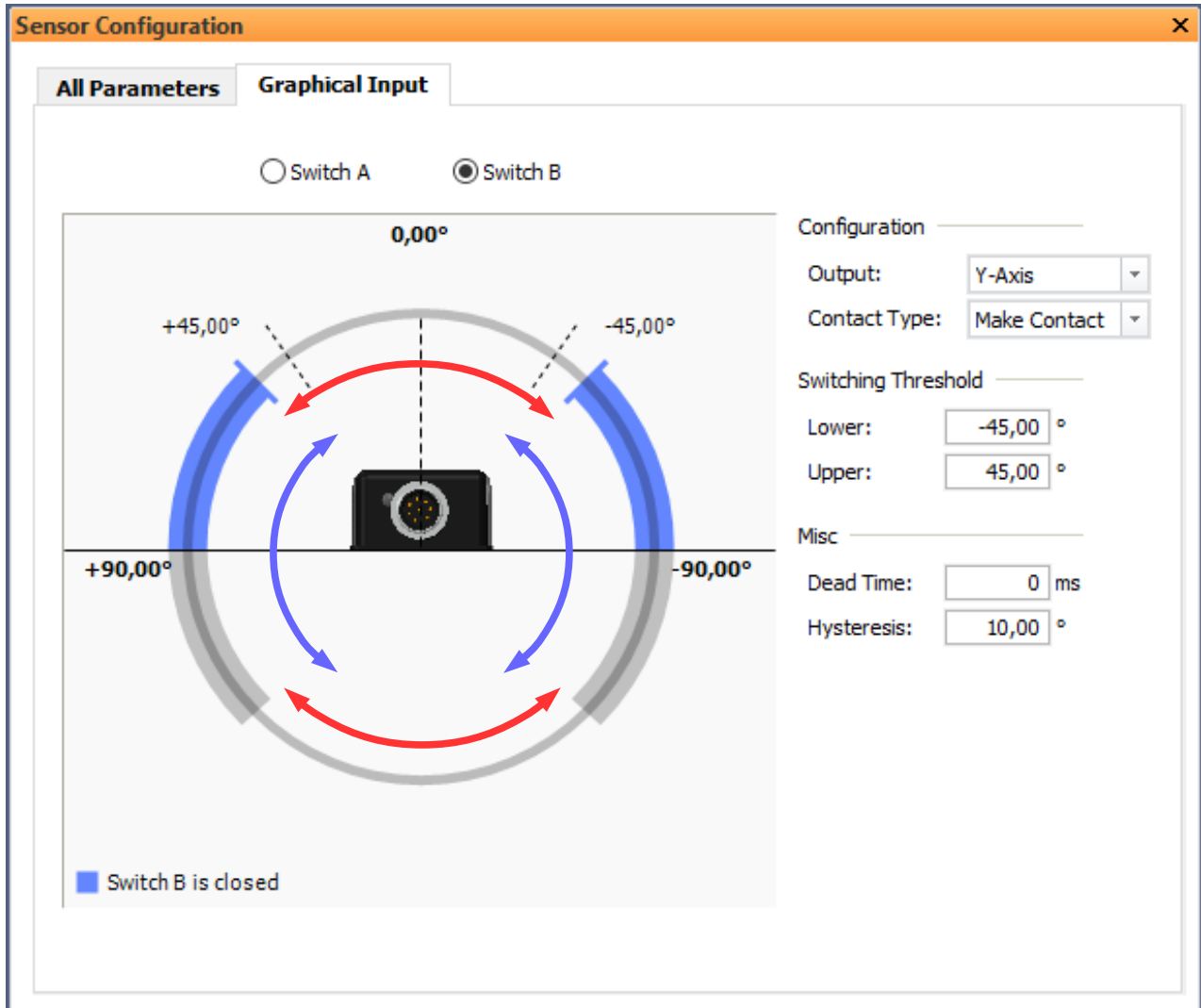
Figure 22: Sensor Configuration Graphical Input – Example for hysteresis of 10^\circ and switching threshold levels of -45^\circ/+45^\circ on the Y-axis (Make Contact)
