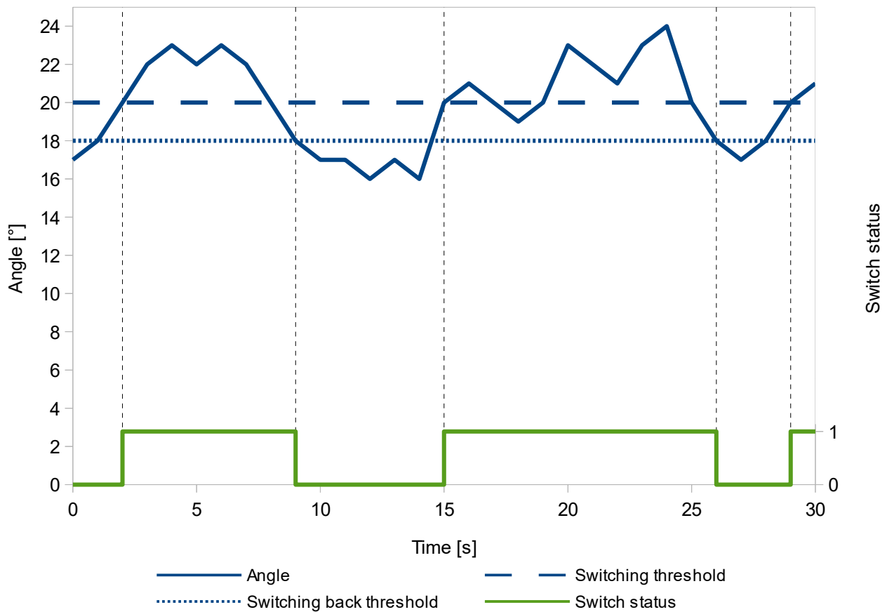
Figure 13: Example hysteresis of 2°
