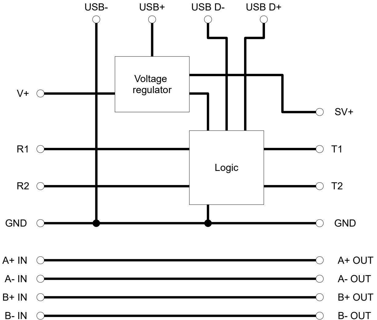
Figure 10: Block diagram ISWPA1
