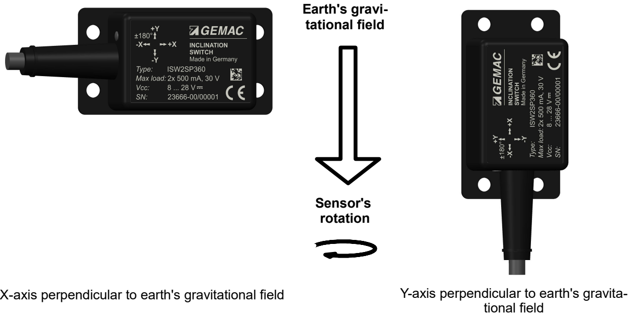
Figure 8: Examples of angle value changes which can not be detected: X-axis (left) and Y-axis (right)
