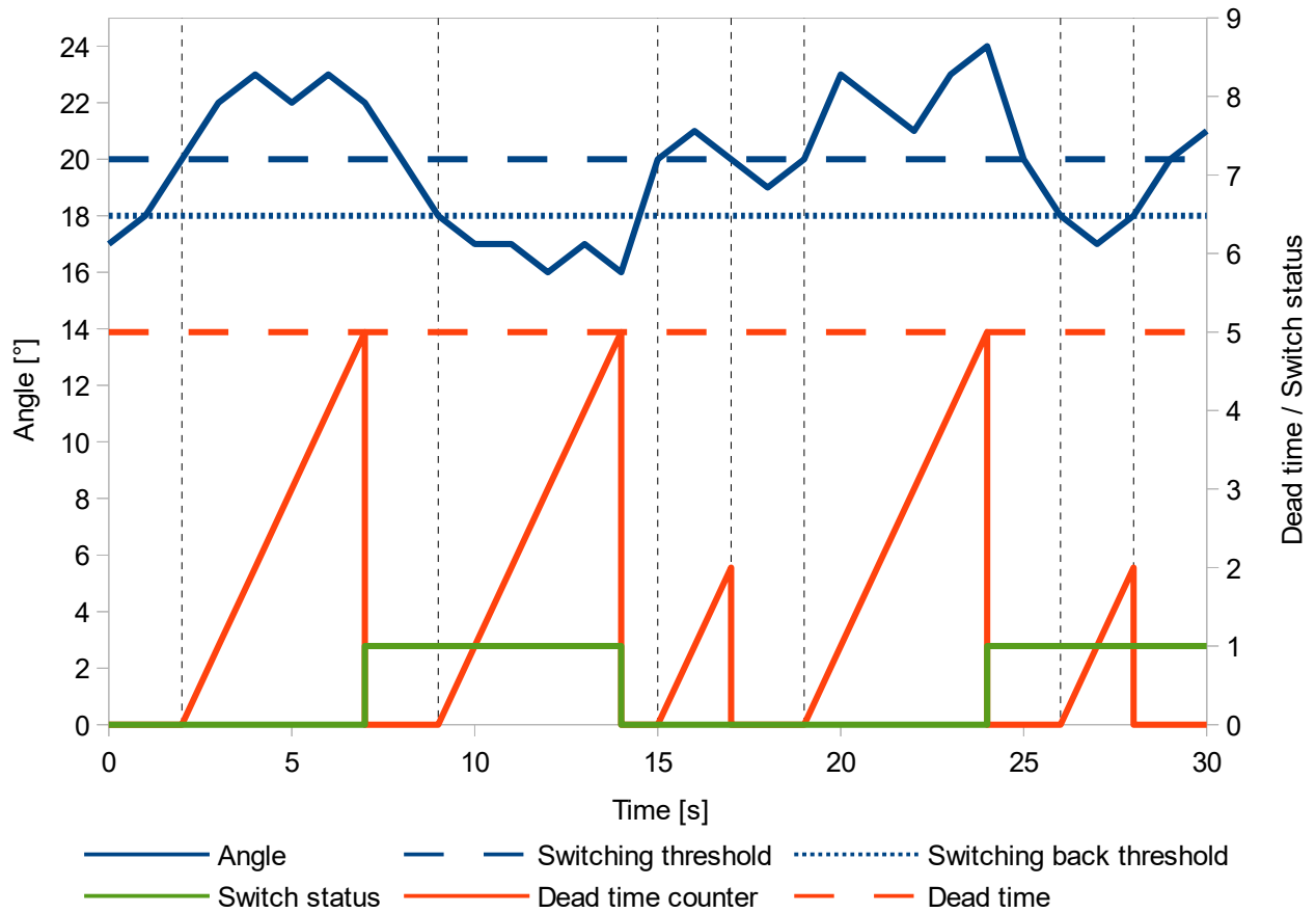
Figure 15: Example hysteresis of 2° and dead time 5 seconds
