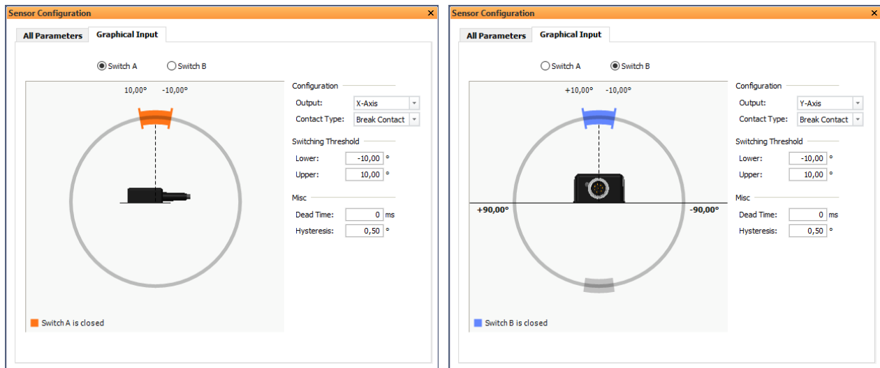
Figure 20: Sensor configuration graphical input
