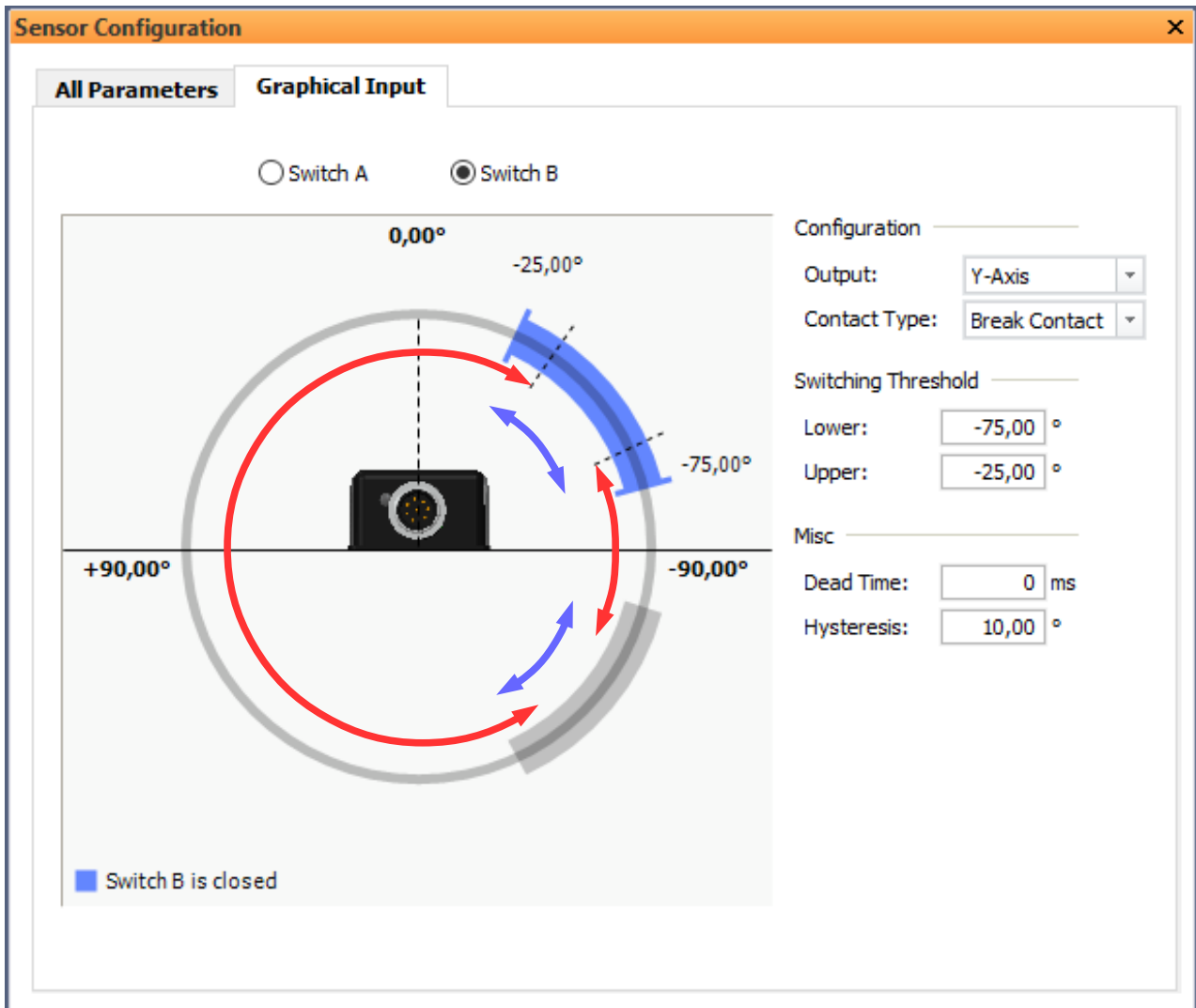
Figure 23: Sensor Configuration Graphical Input – Example for hysteresis of 10° and switching threshold levels of -75°/-25° on the Y-axis (Break Contact)
