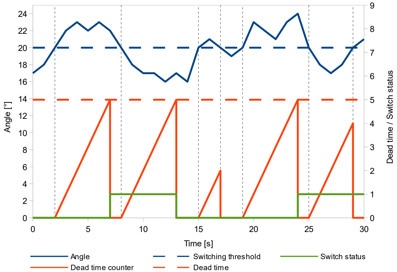
Figure 14: Example hysteresis of 5 seconds
