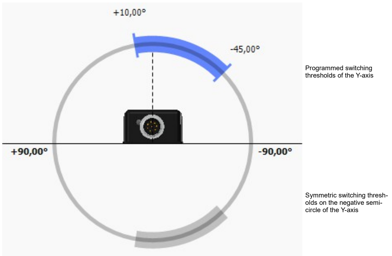
Figure 7: Switching thresholds of the Y-axis
