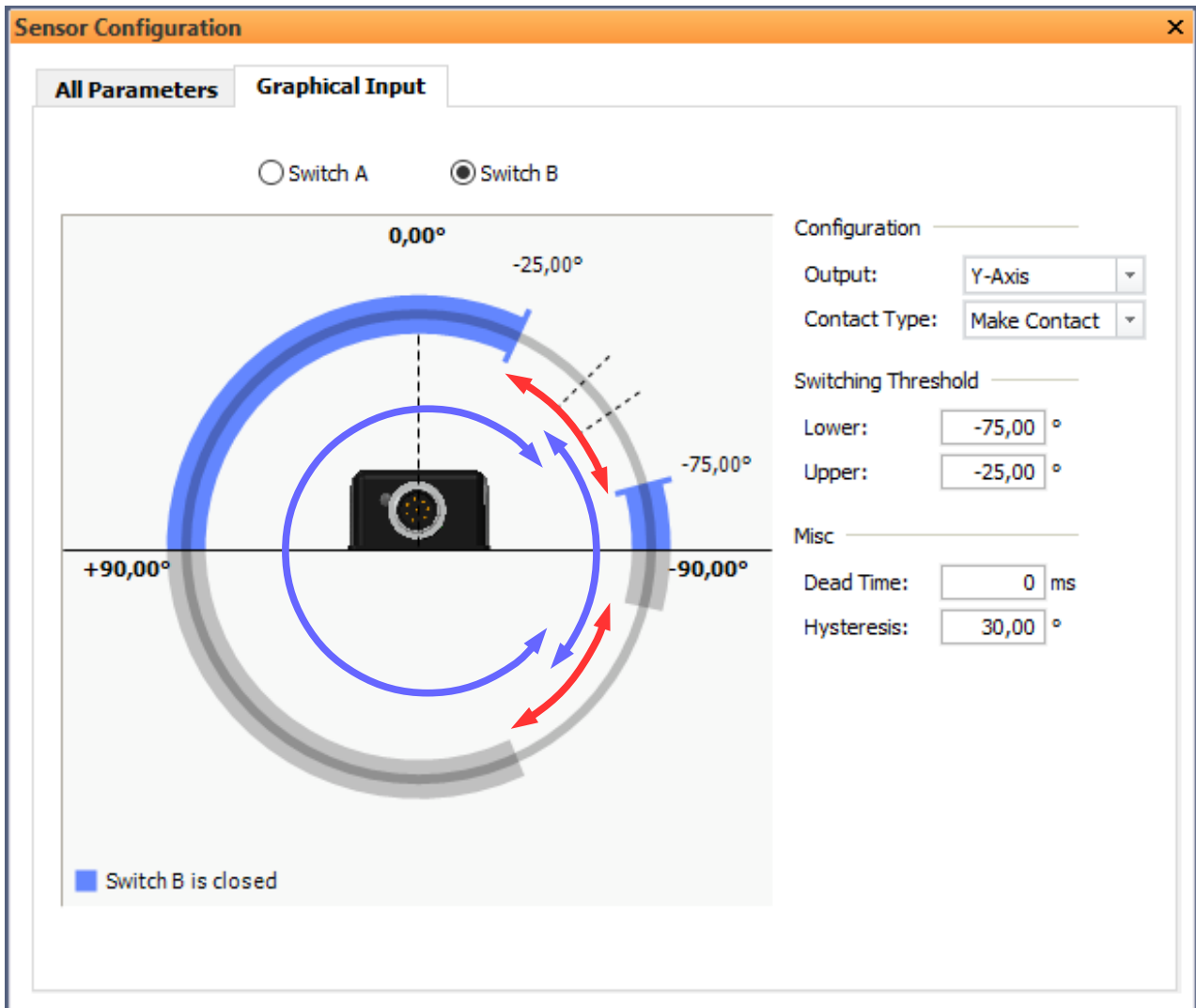
Figure 24: Sensor Configuration Graphical Input – Example for hysteresis of 30° and switching threshold levels of -75°/-25° on the Y-axis (Make Contact)
