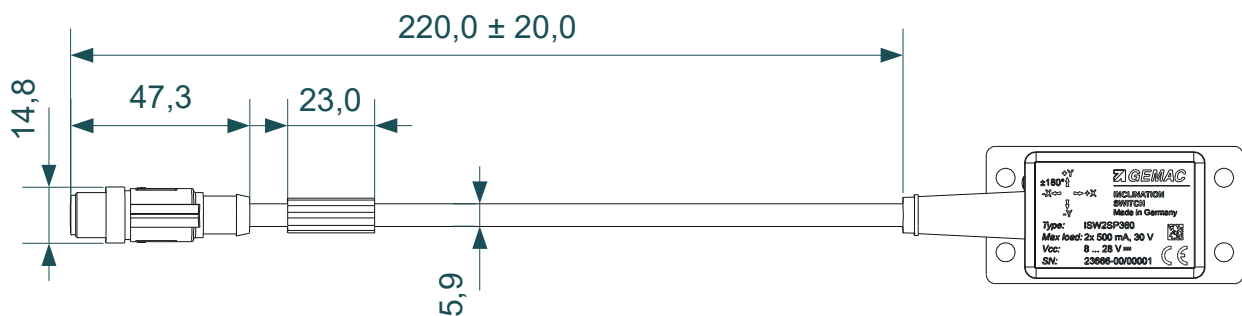
Figure 4: Dimensioned drawing ISW2SP360 (dimensions in mm)
