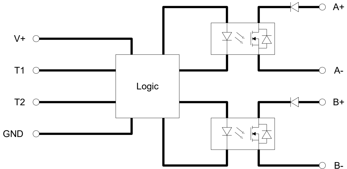
Figure 3: Block diagram ISW2SP360
