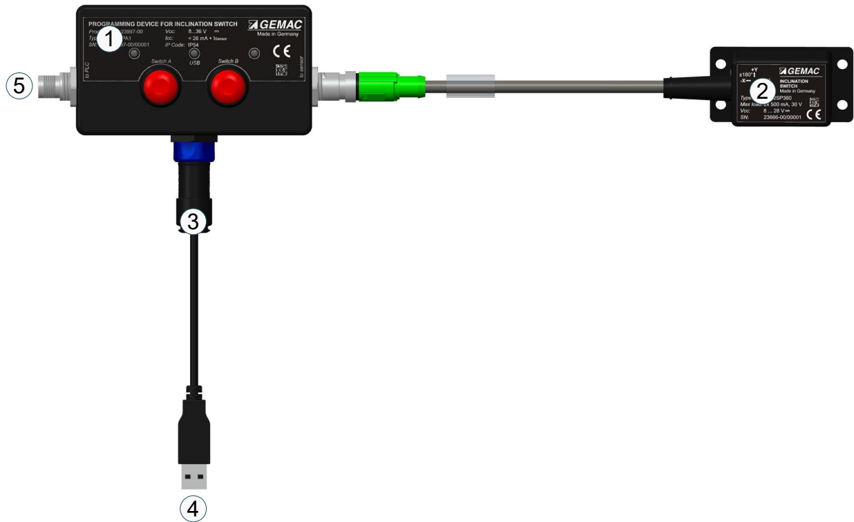
Figure 16: Connecting programming device and inclinations switch with a computer
