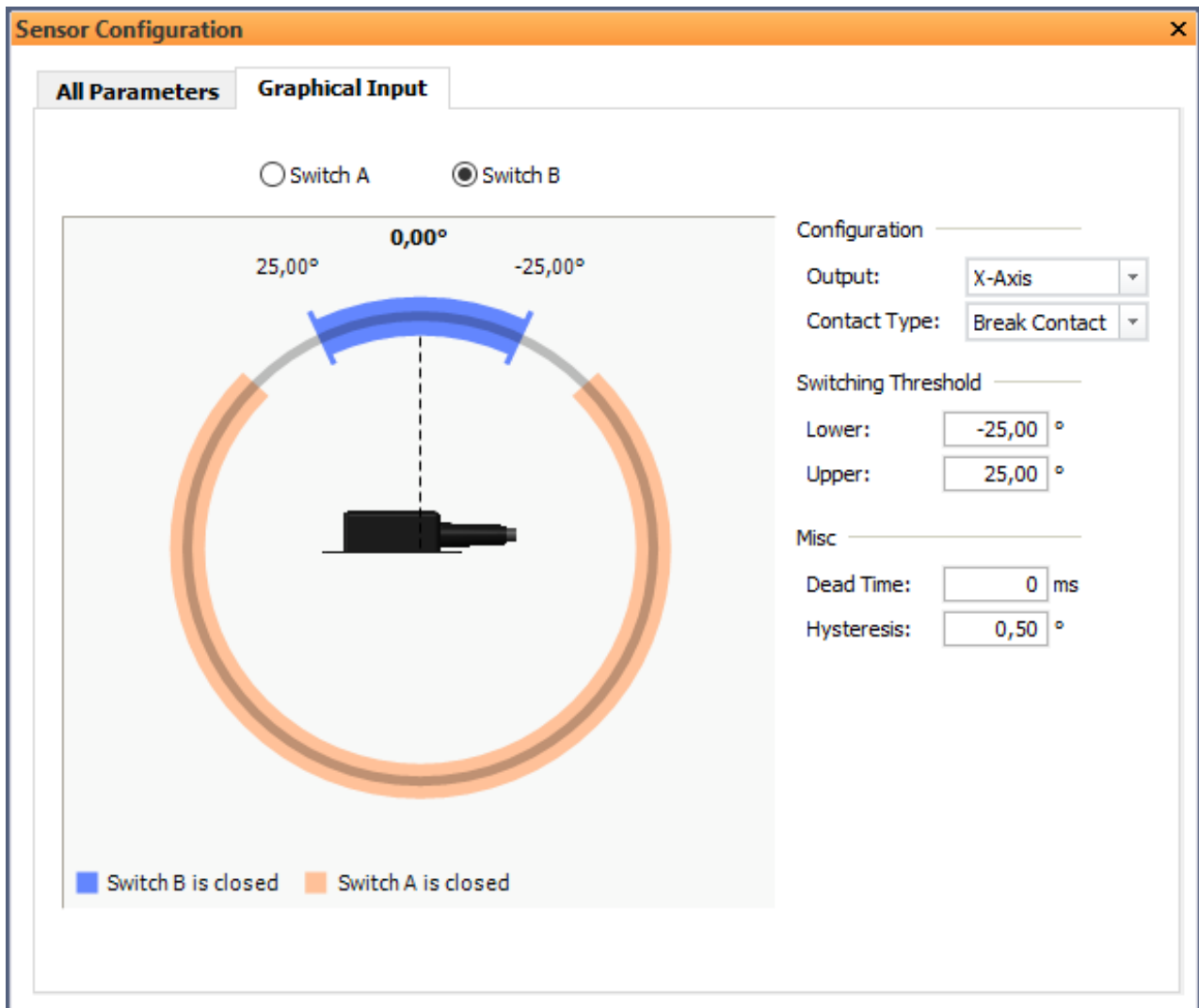
Figure 21: Sensor configuration graphical input – example for relation of X-axis to both switching outputs
